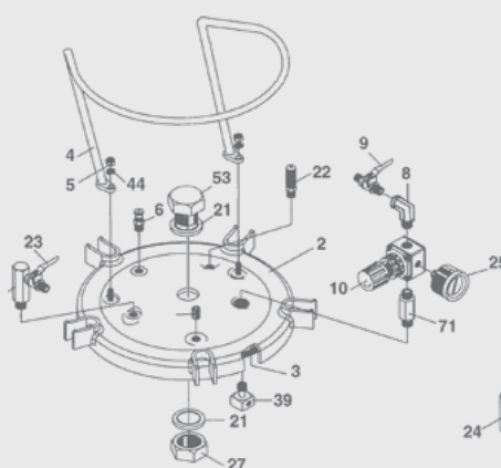
Model N : Version without PNEUMATIC AGITATOR
