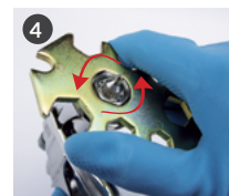
Unscrew the fluid nozzle with universal spanner (code 930171A0).
