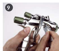
Adjust (15-60 degree tighten) the needle packing with spanner.
