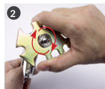
Tighten up the fluid nozzle with the universal spanner (code 930171A0).
