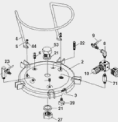
Model N: Version without PNEUMATIC AGITATOR
